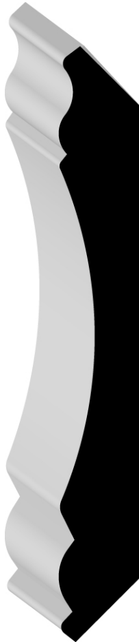
Crown 05982-H 5/8 X 4.1/2 Information Page 4
