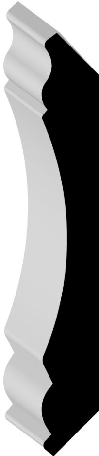
Crown 05982-9 5/8 X 4.1/2 Information Page 4
